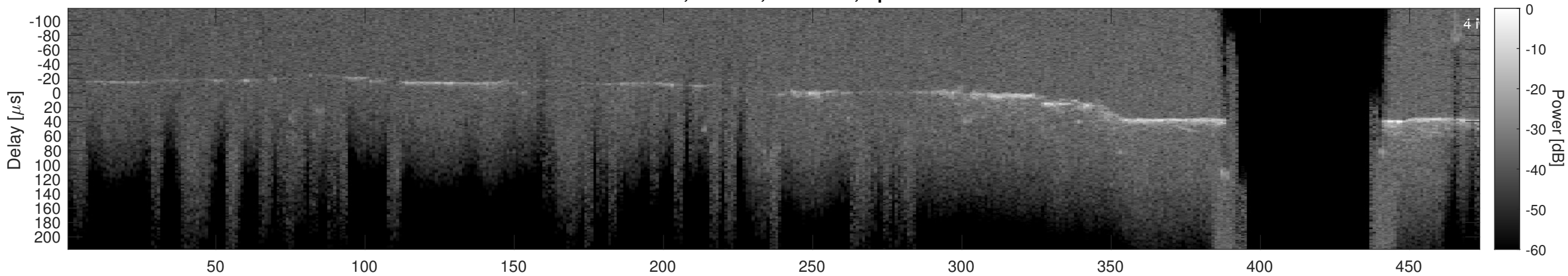
Orbit 3135, Cluttergram
