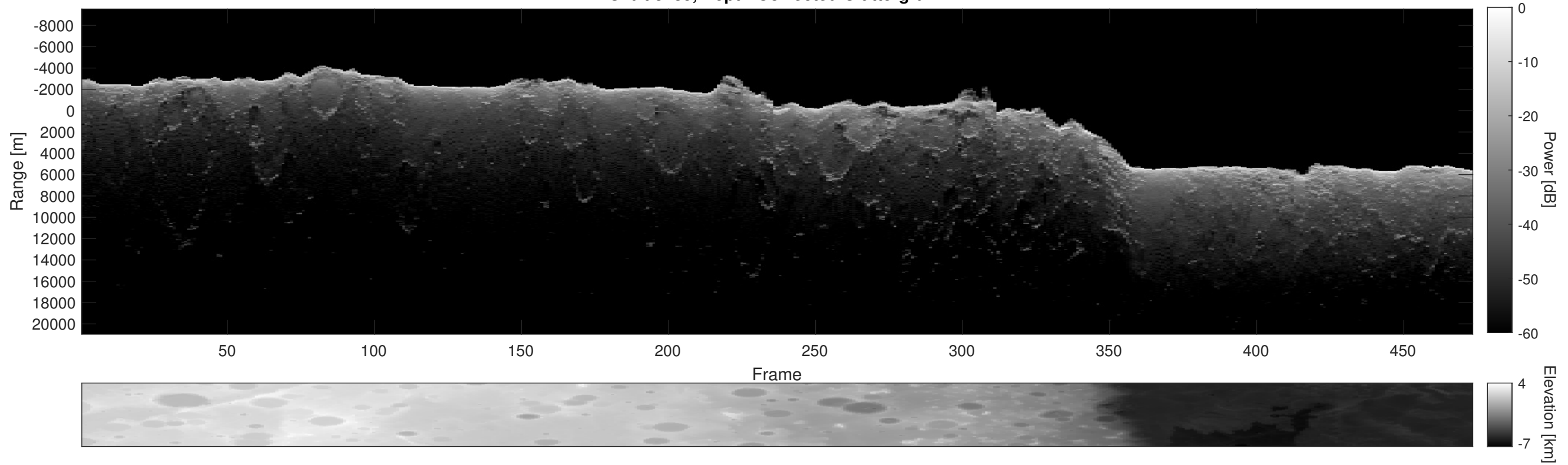
Orbit 3135, Depth-Corrected Cluttergram
