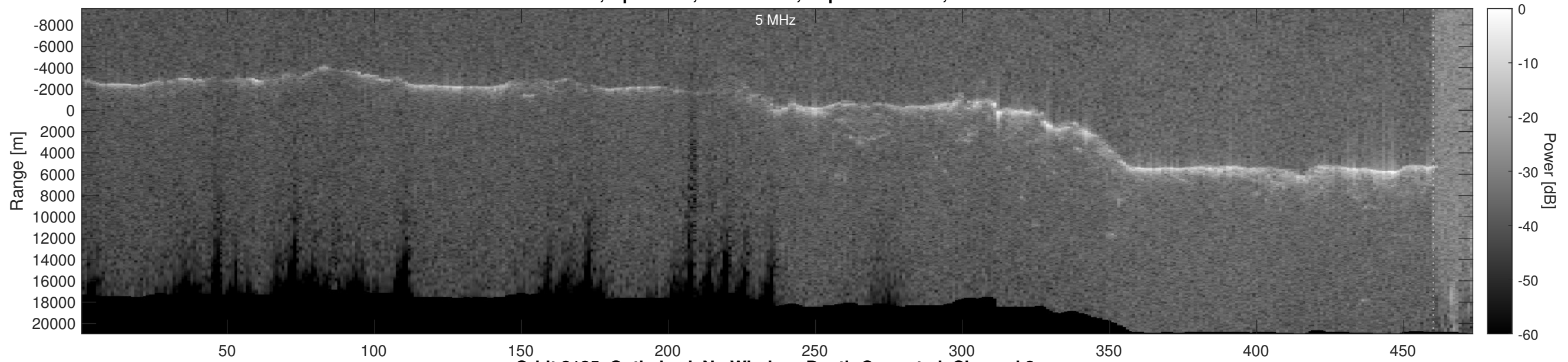
Orbit 3135, Optimized, No Window, Depth-Corrected, Channel 2
