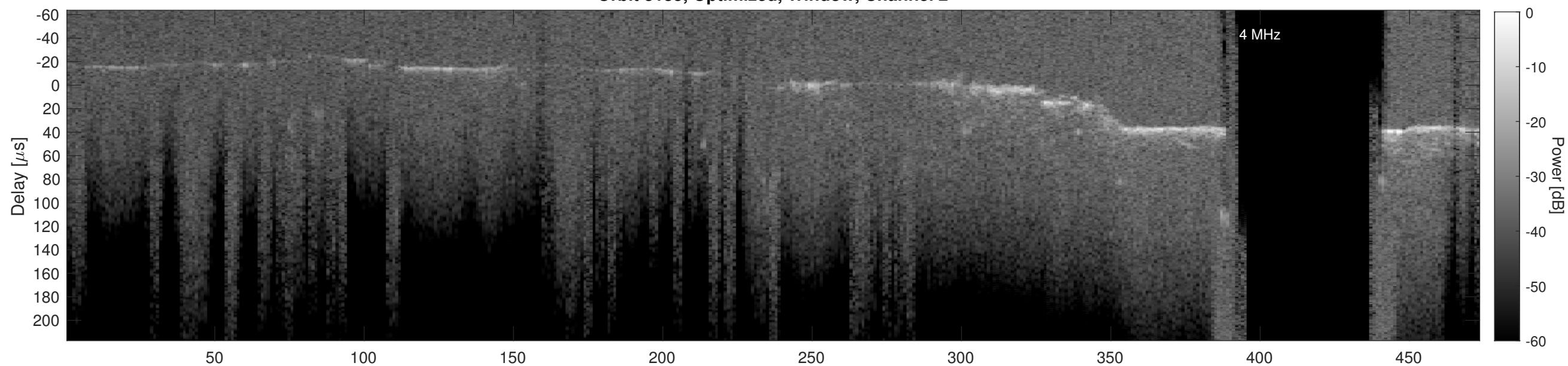
Orbit 3135, Cluttergram
