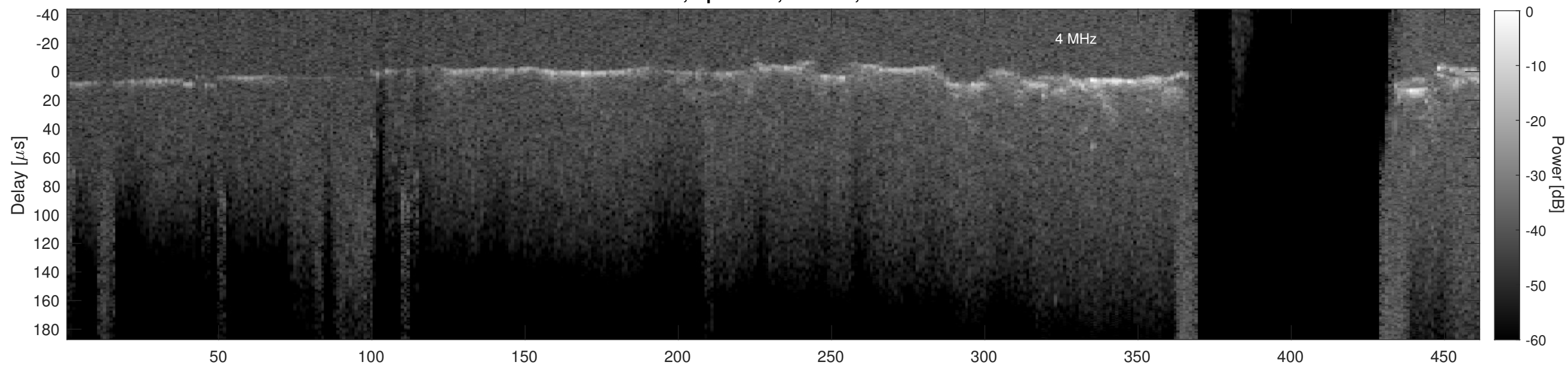
Orbit 3139, Cluttergram
