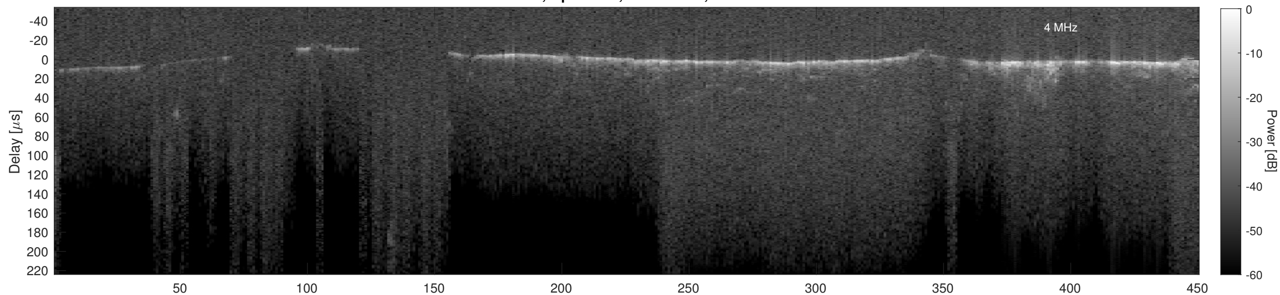
Orbit 3140, Cluttergram
