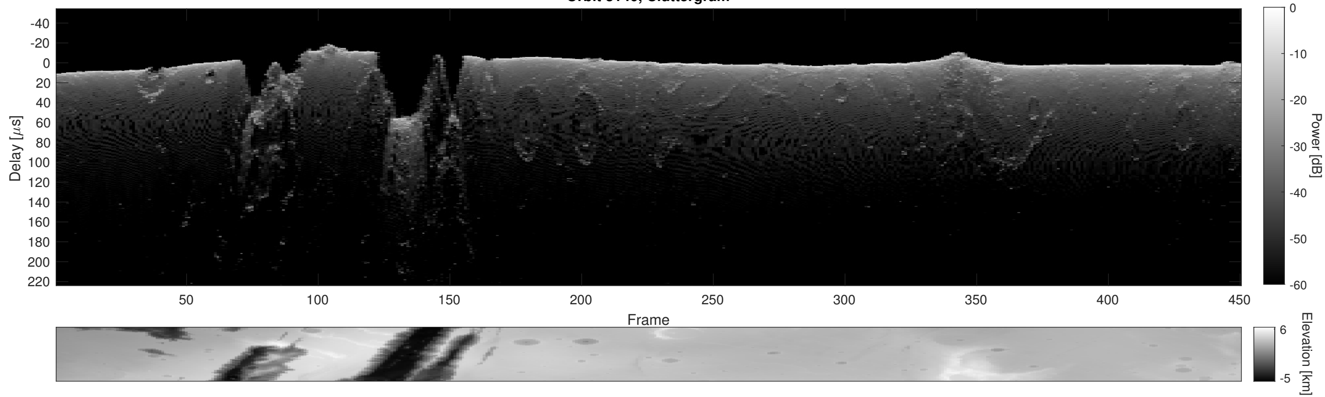
Orbit 3140, Cluttergram
