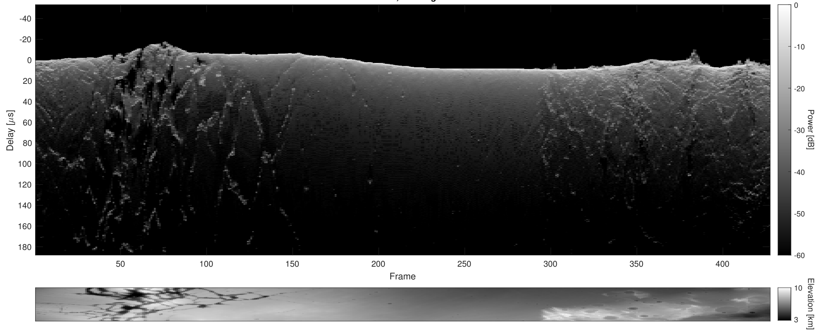
Orbit 3144, Cluttergram
