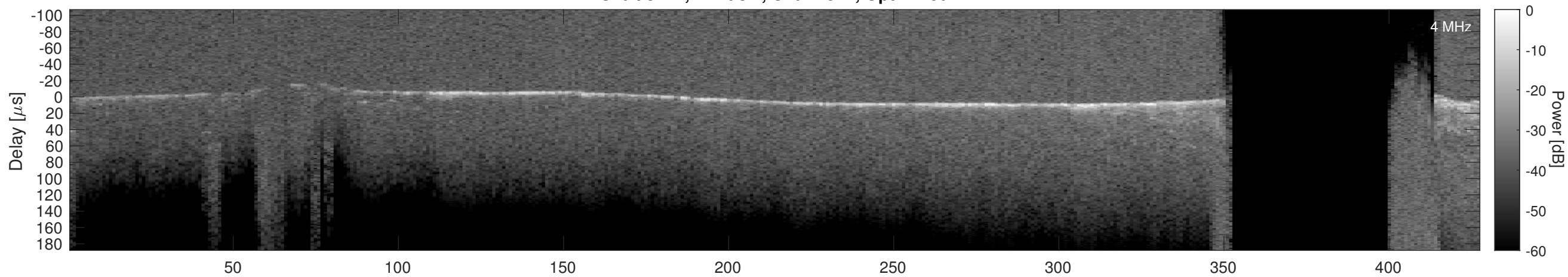
Orbit 3144, Cluttergram
