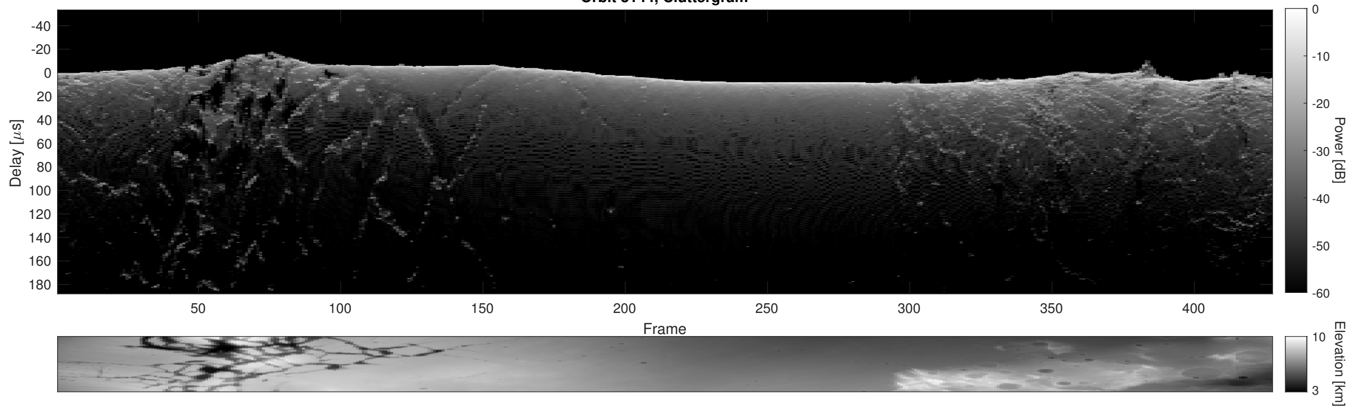
Orbit 3144, Cluttergram
