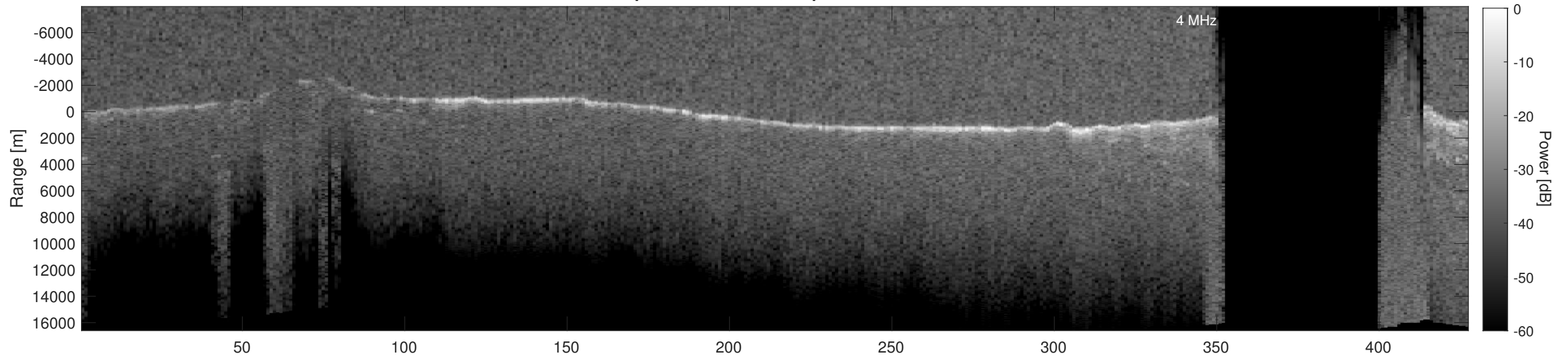
Orbit 3144, Depth-Corrected Cluttergram
