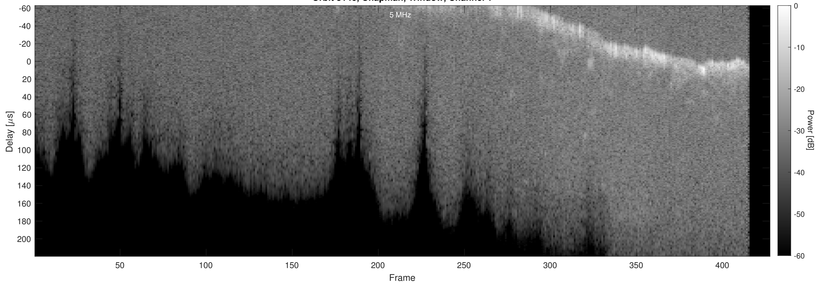
Orbit 3146, Chapman, Window, Channel 2
