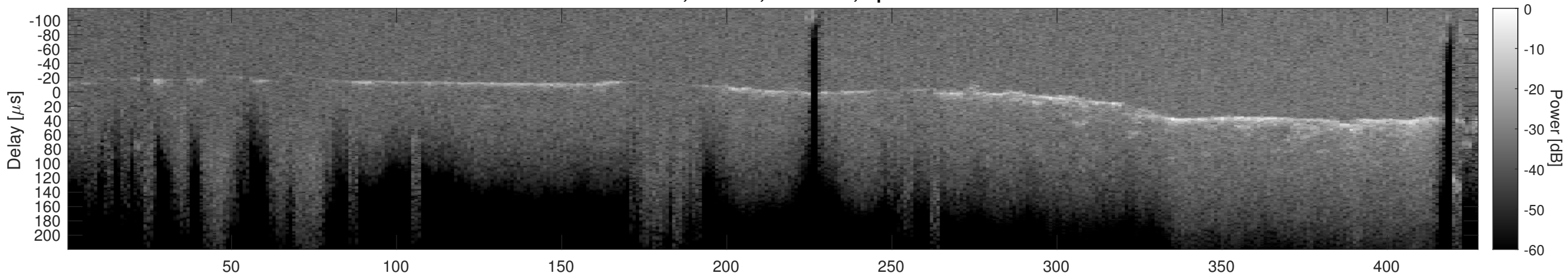
Orbit 3146, Cluttergram
