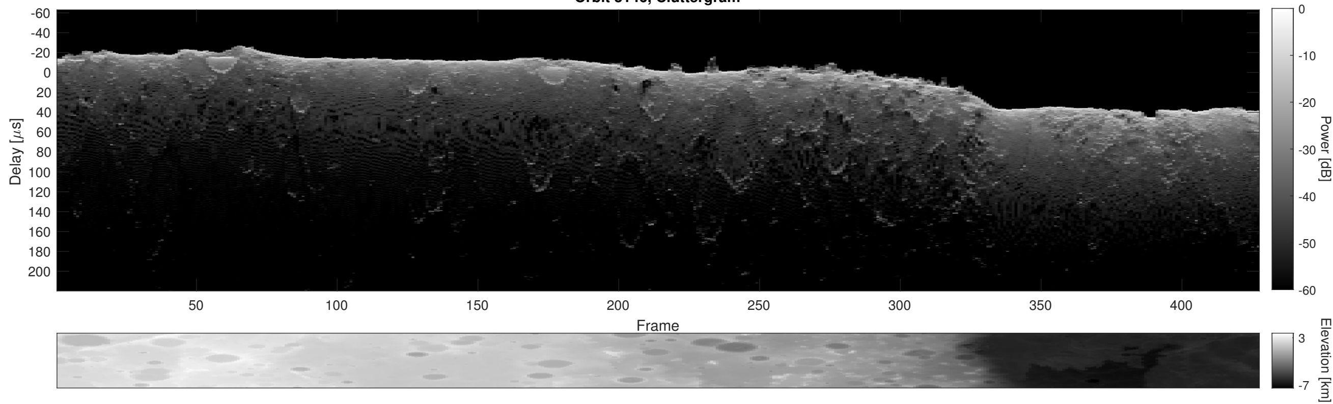
Orbit 3146, Cluttergram
