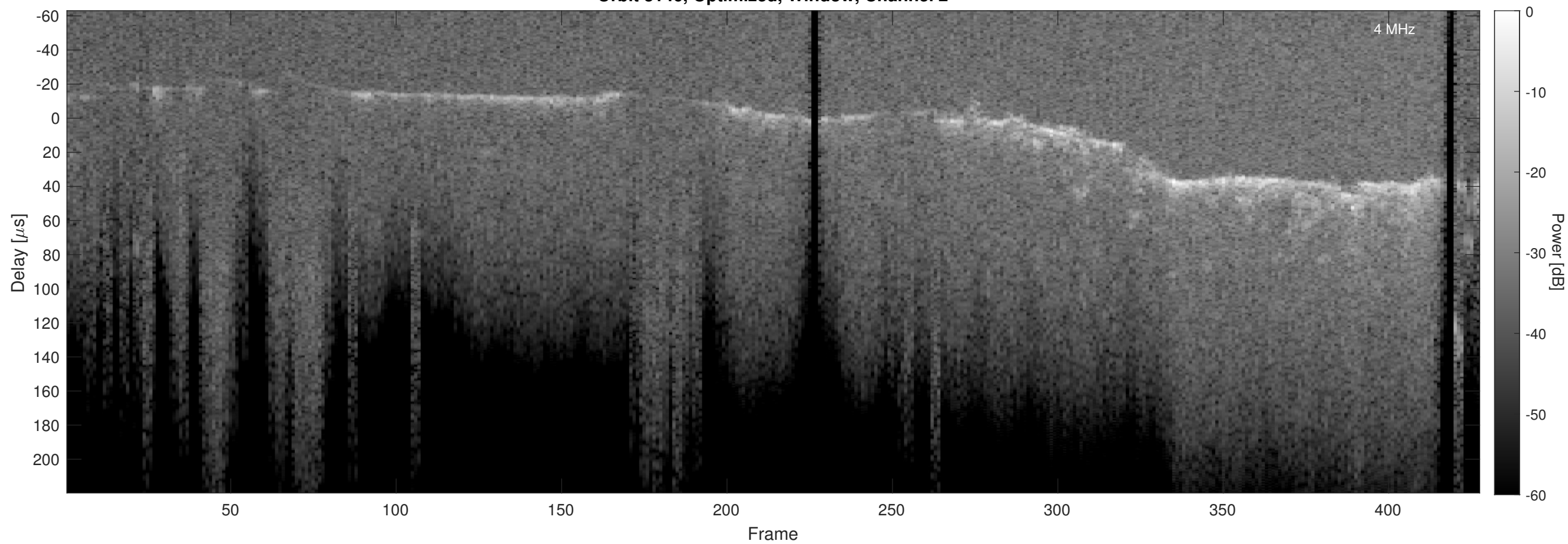
Orbit 3146, Optimized, Window, Channel 2
