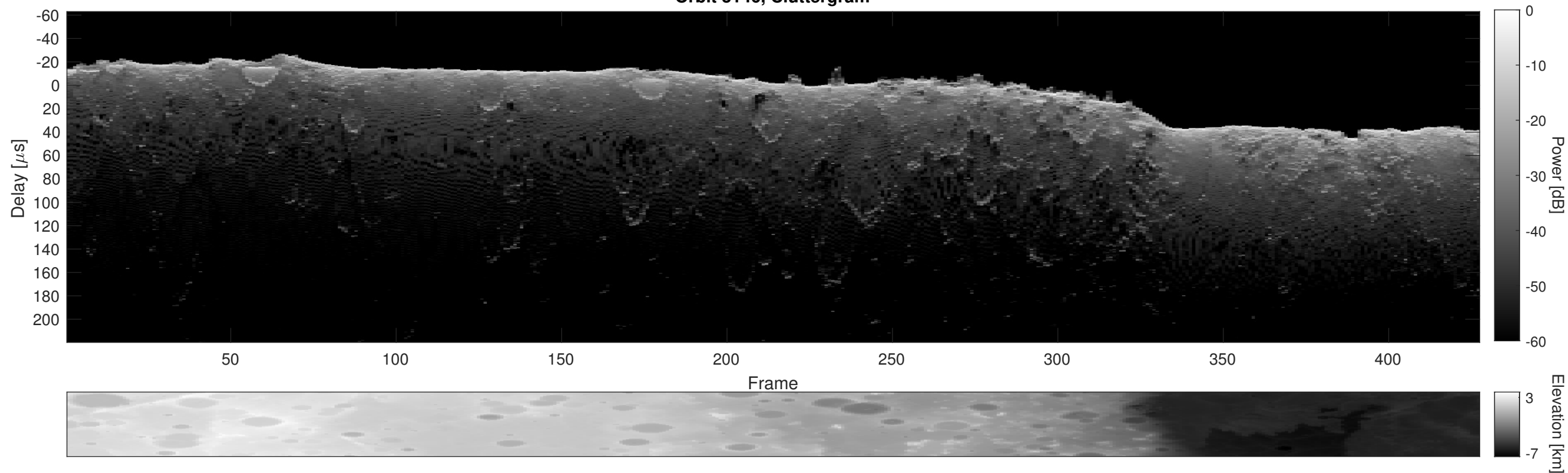
Orbit 3146, Cluttergram
