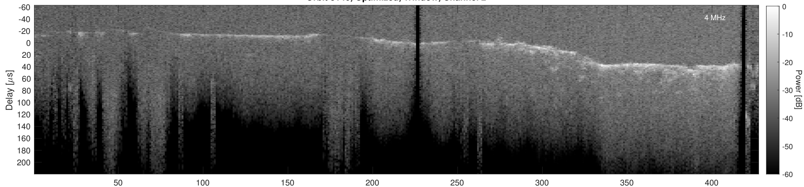
Orbit 3146, Cluttergram
