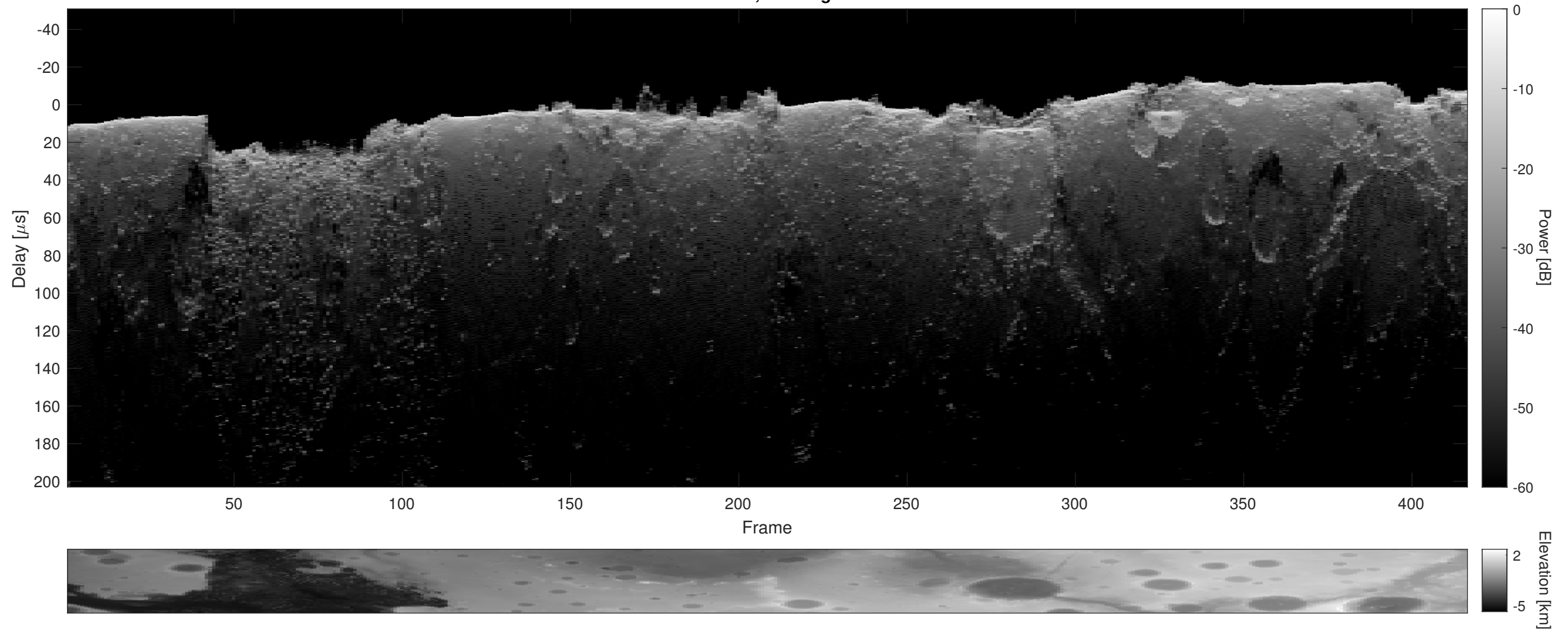
Orbit 3147, Cluttergram
