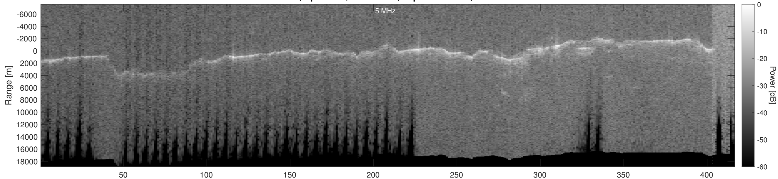
Orbit 3147, Optimized, No Window, Depth-Corrected, Channel 2
