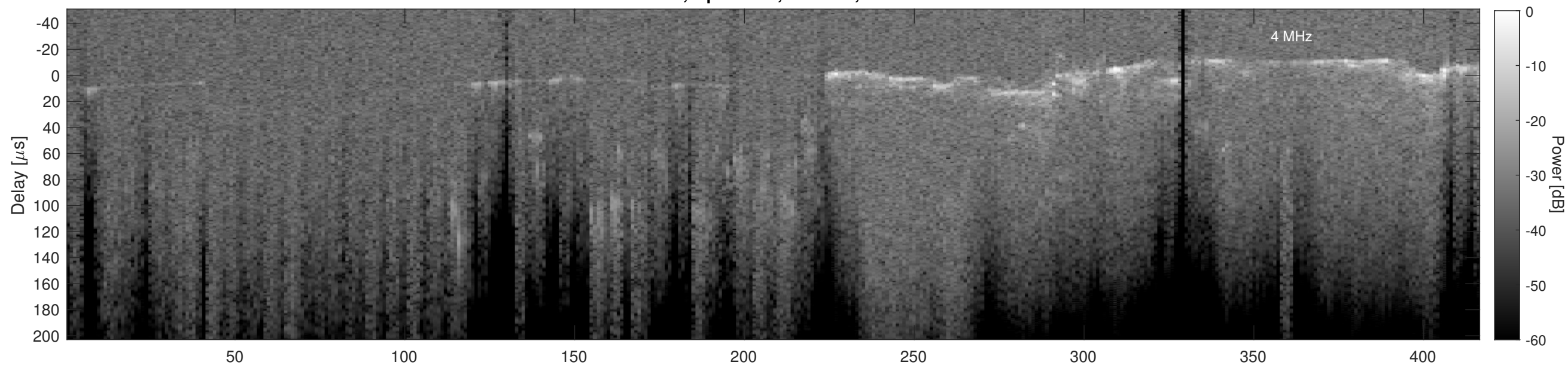
Orbit 3147, Cluttergram
