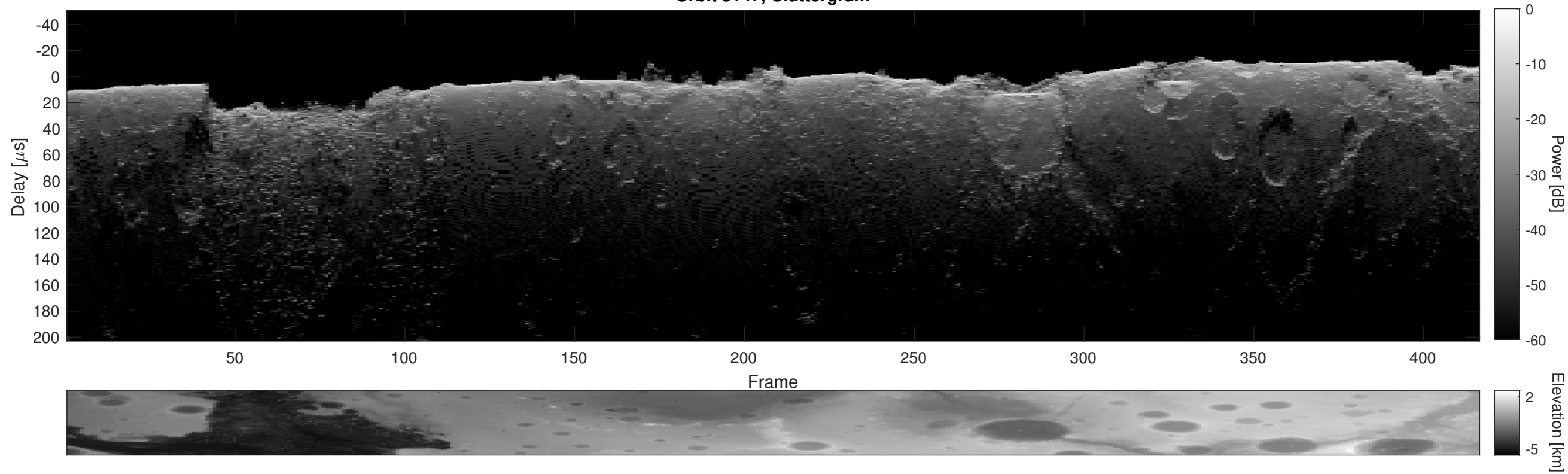
Orbit 3147, Cluttergram
