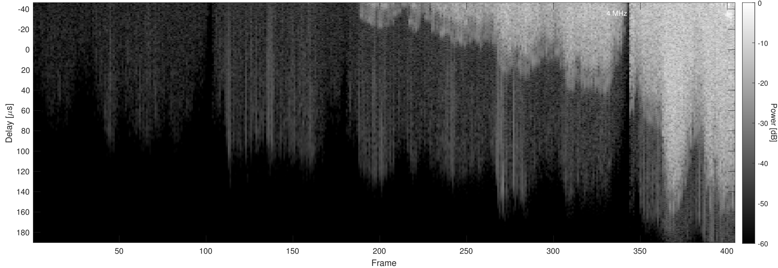
Orbit 3149, Chapman, No Window, Channel 2
