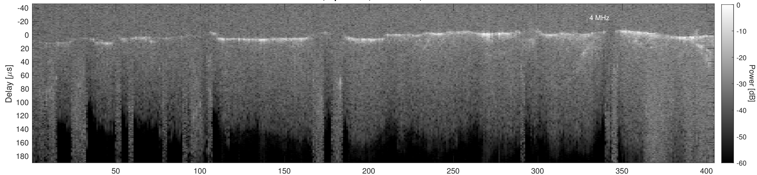
Orbit 3149, Cluttergram
