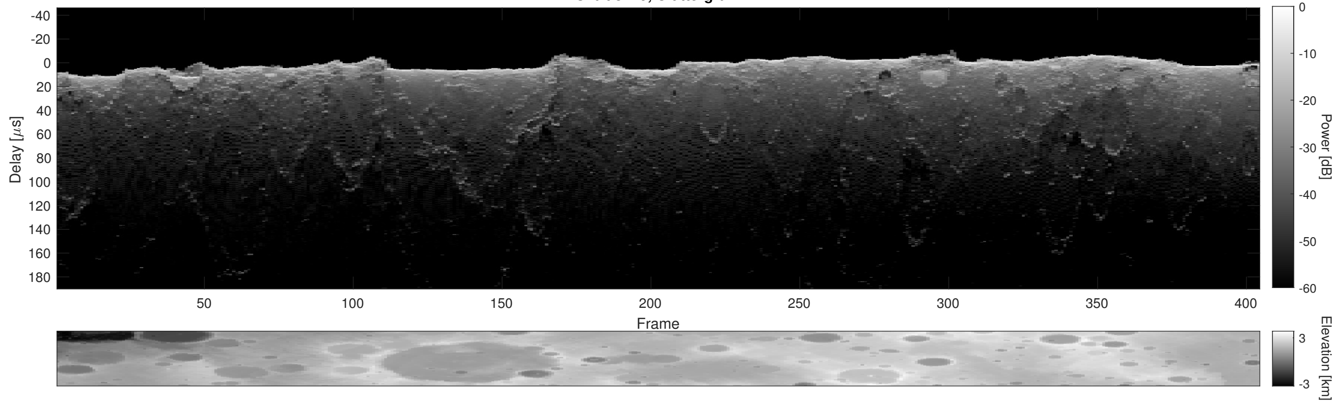
Orbit 3149, Cluttergram
