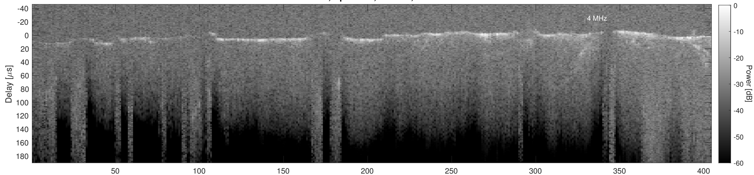
Orbit 3149, Cluttergram
