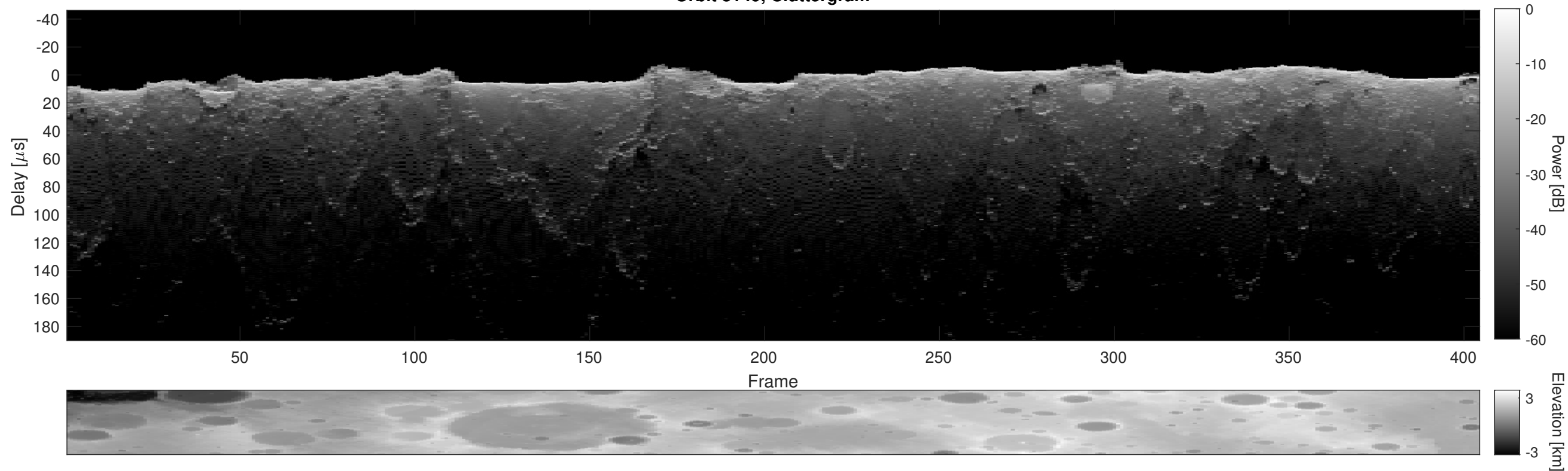
Orbit 3149, Cluttergram
