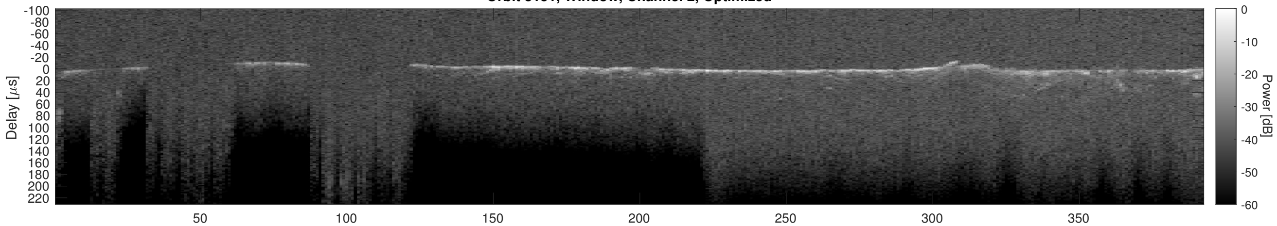
Orbit 3151, Cluttergram
