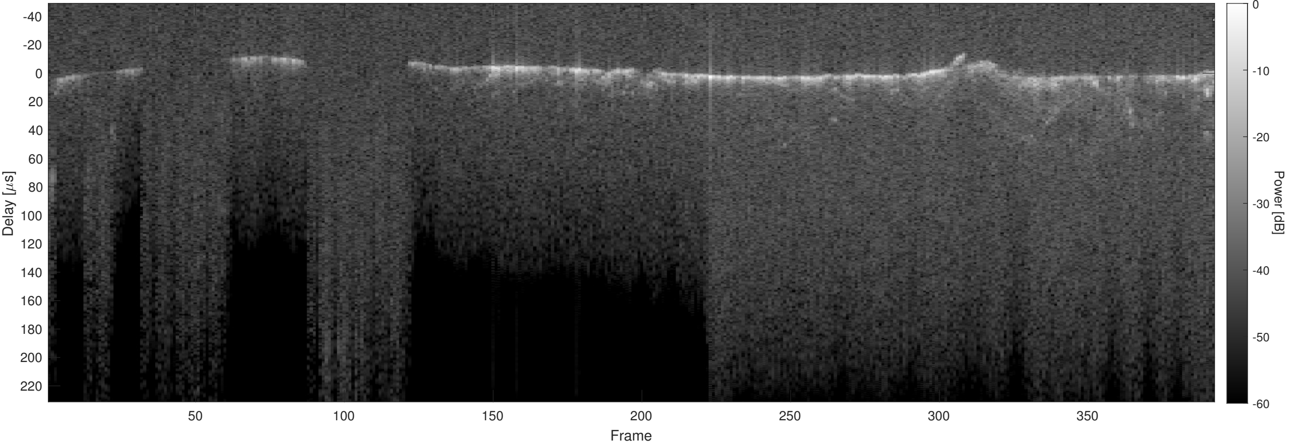
Orbit 3151, Optimized, No Window, Channel 2
