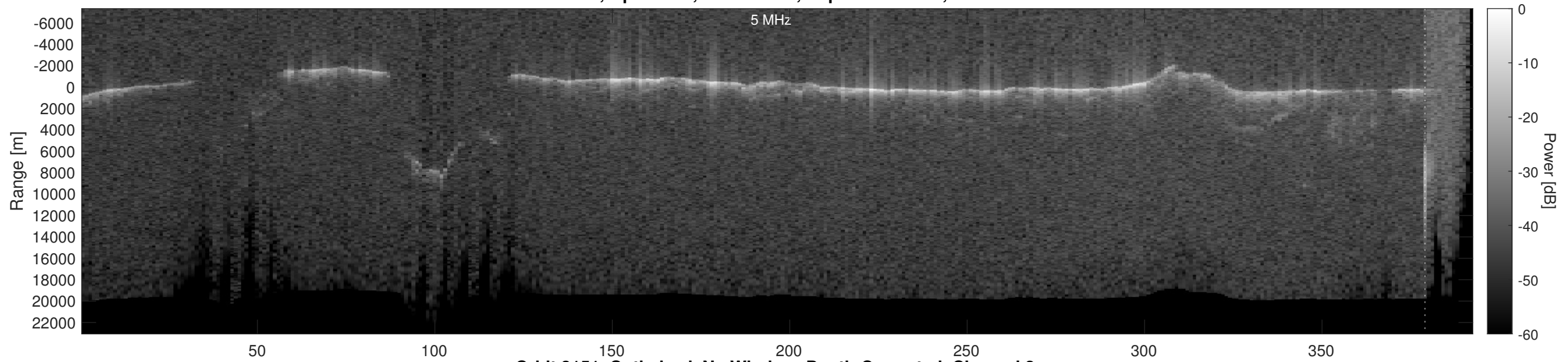
Orbit 3151, Optimized, No Window, Depth-Corrected, Channel 2
