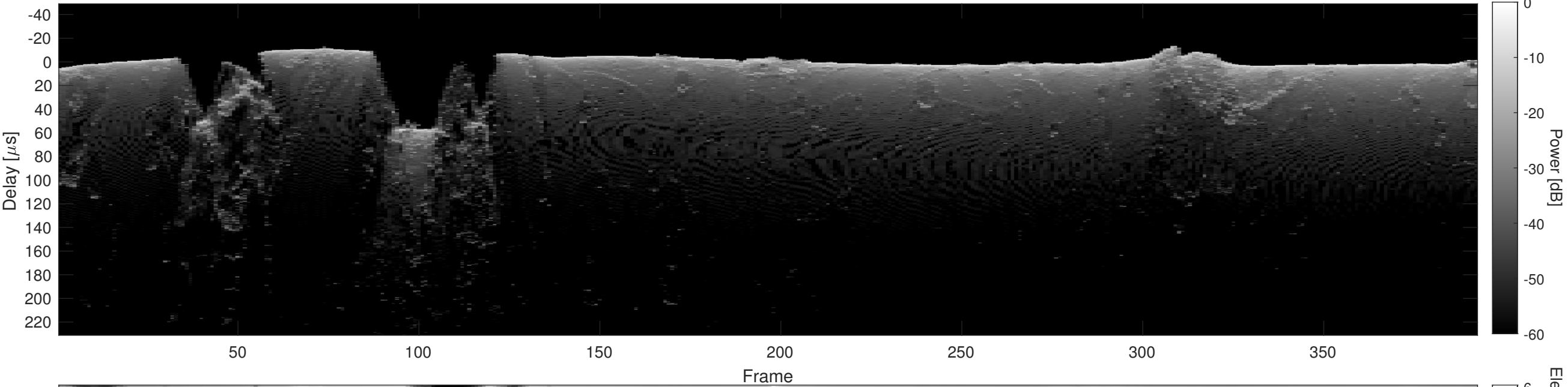
Orbit 3151, Cluttergram
