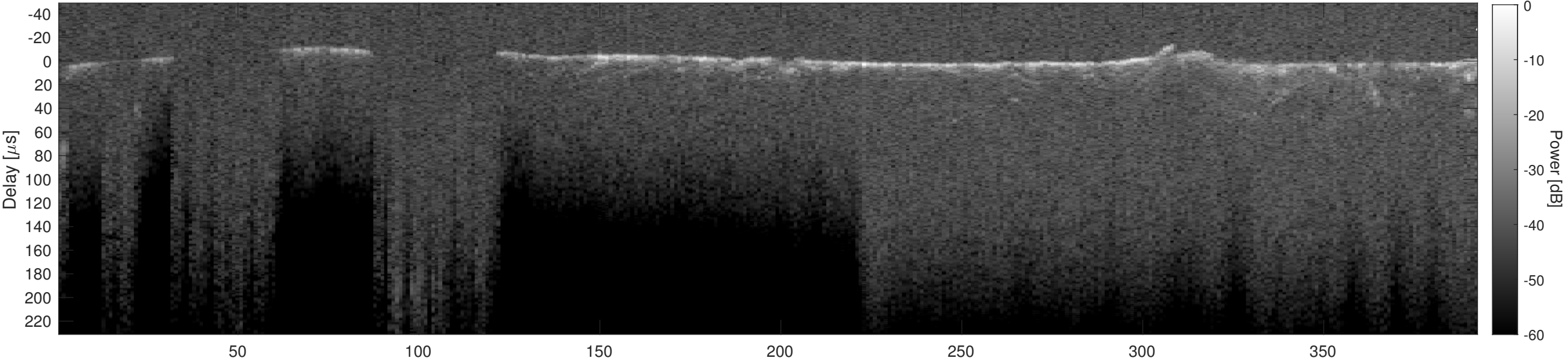
Orbit 3151, Cluttergram
