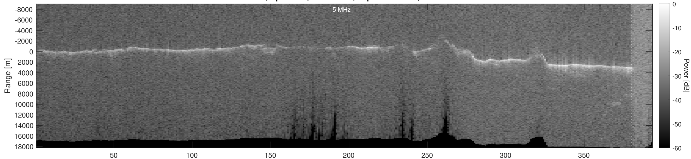
Orbit 3153, Optimized, No Window, Depth-Corrected, Channel 2
