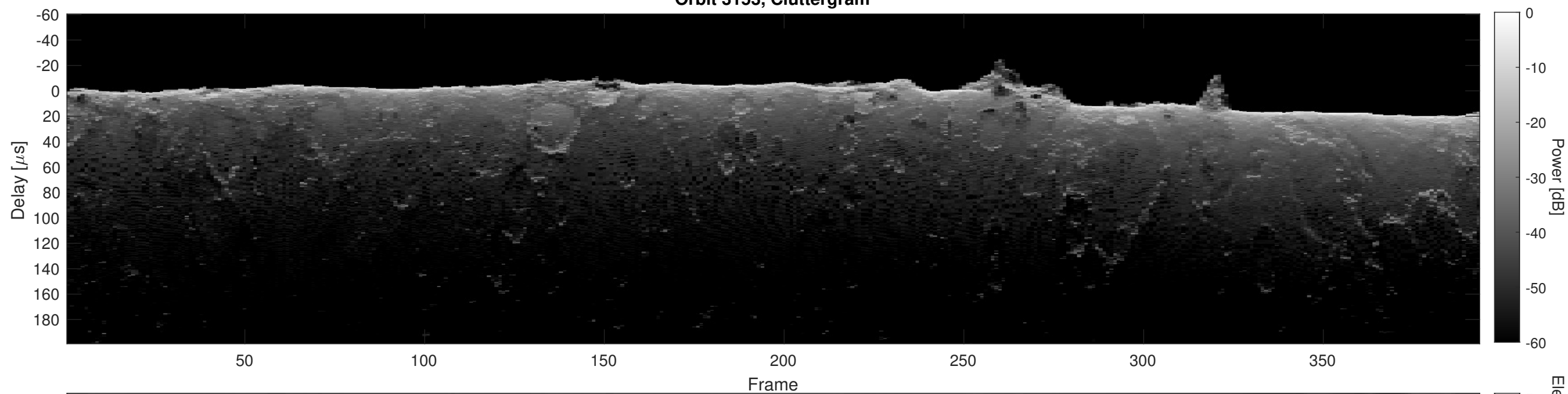
Orbit 3153, Cluttergram
