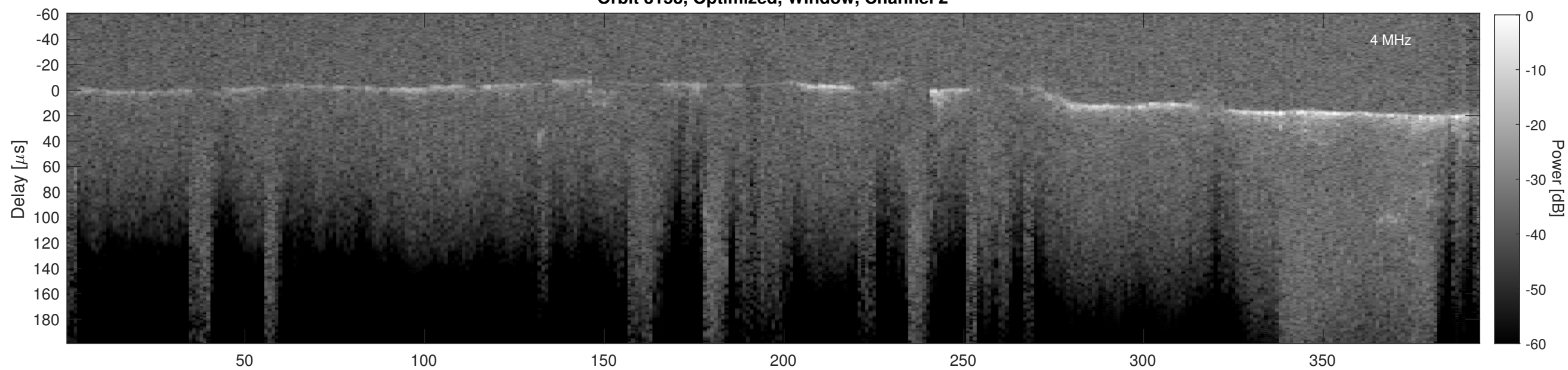
Orbit 3153, Cluttergram
