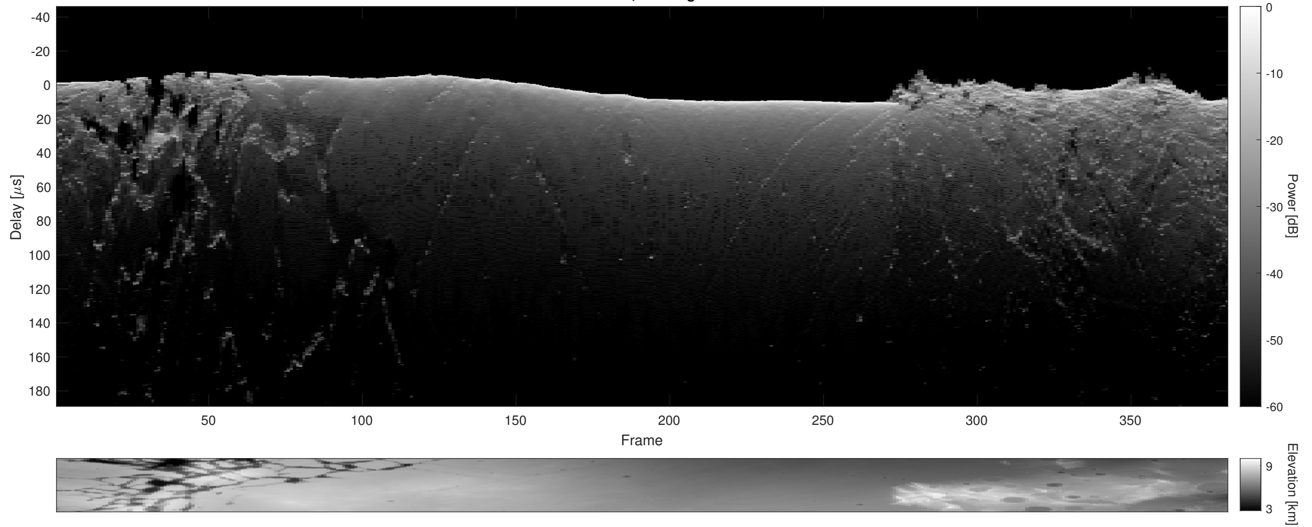
Orbit 3155, Cluttergram
