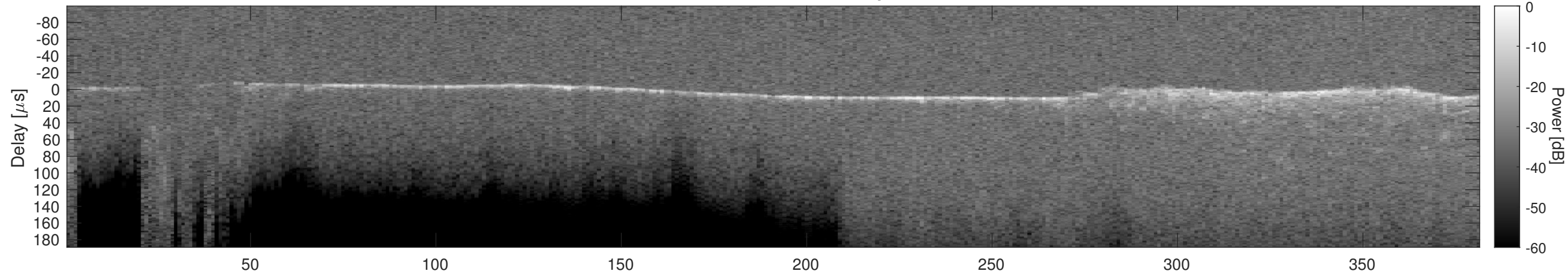
Orbit 3155, Cluttergram
