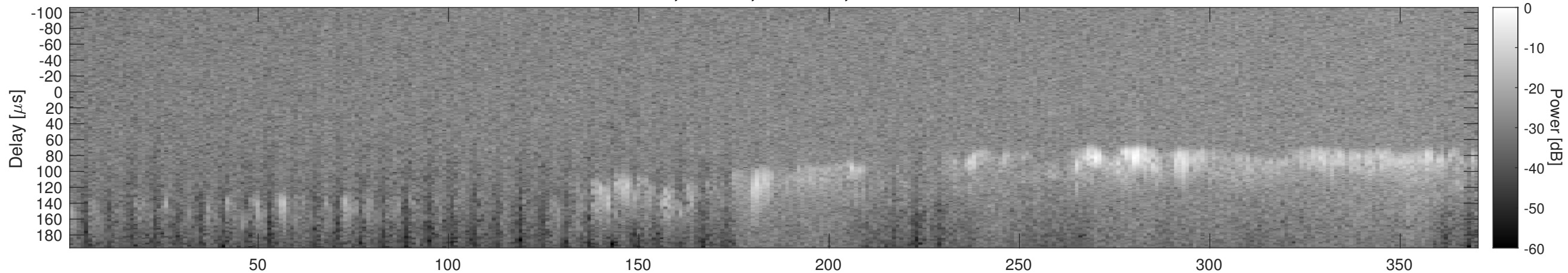
Orbit 3156, Window, Channel 2, Chapman
