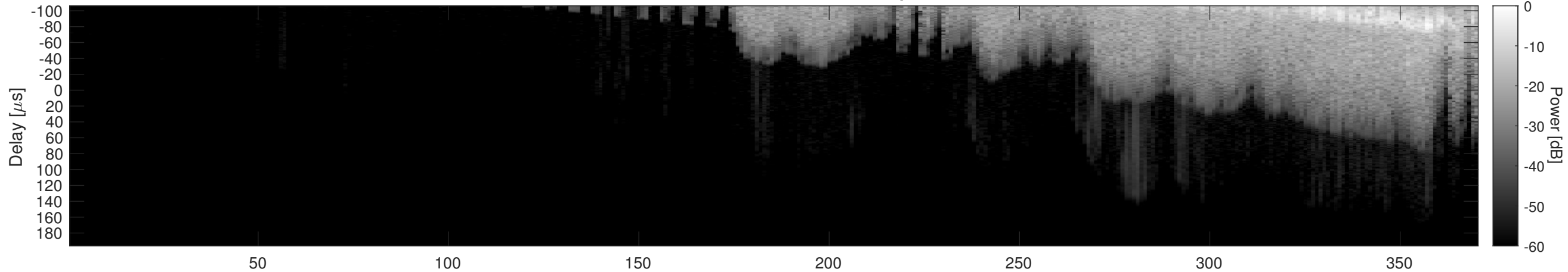
Orbit 3156, Window, Channel 2, Optimized
