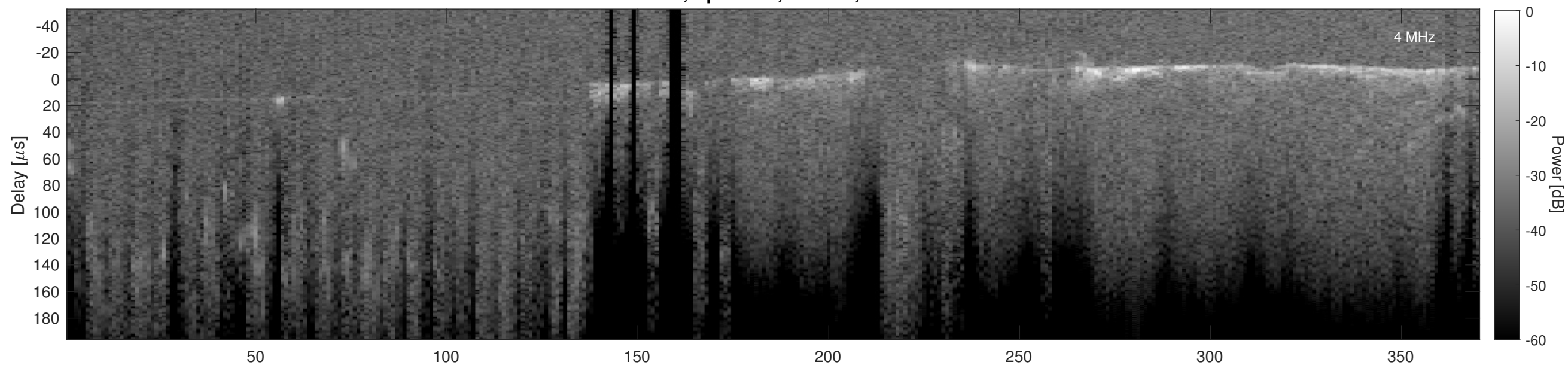
Orbit 3156, Cluttergram
