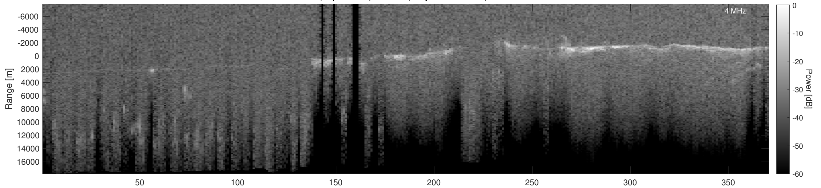
Orbit 3156, Depth-Corrected Cluttergram
