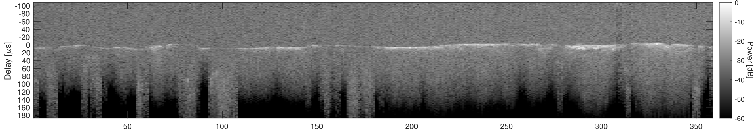
Orbit 3160, Cluttergram
