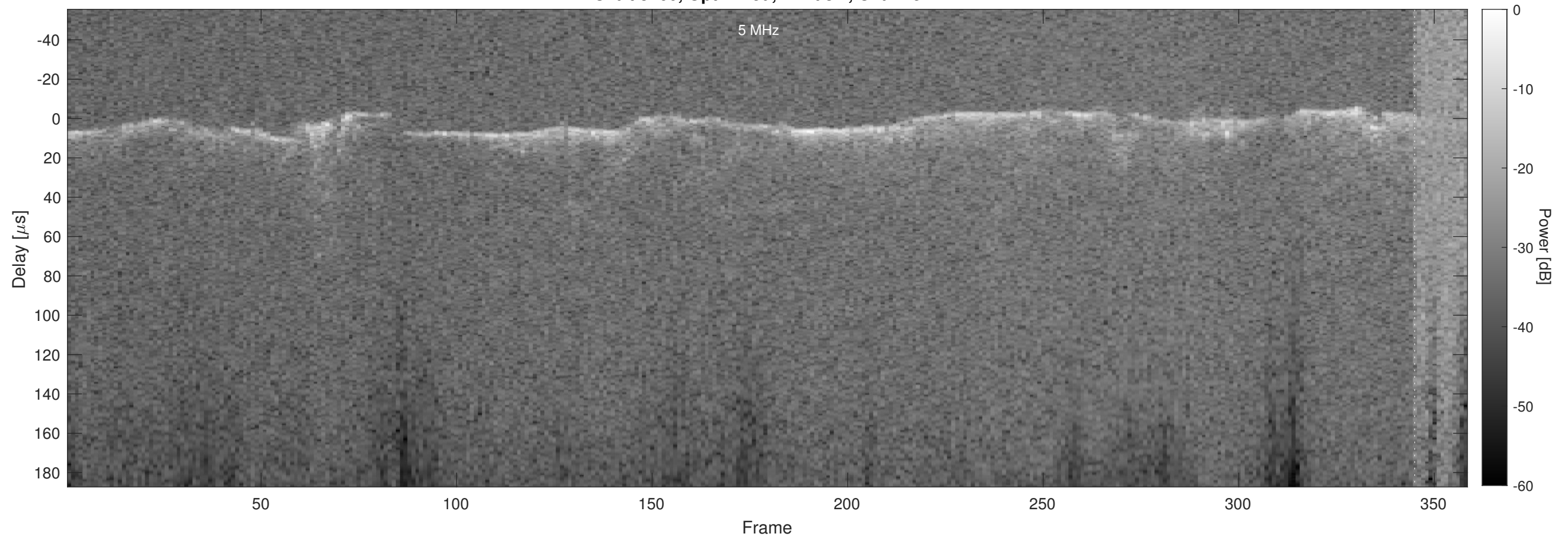
Orbit 3160, Optimized, Window, Channel 2
