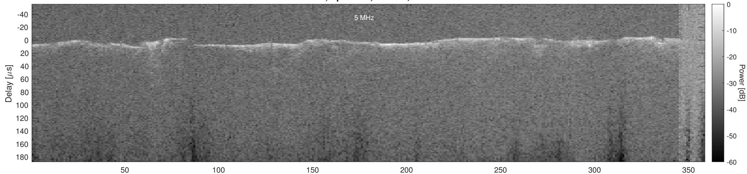
Orbit 3160, Optimized, Window, Channel 2
