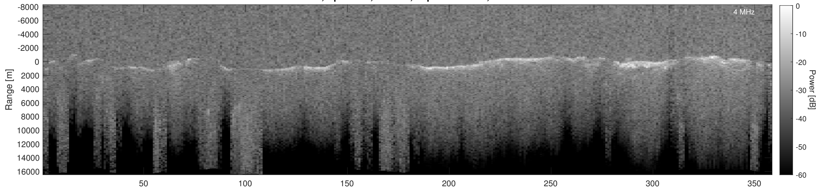
Orbit 3160, Depth-Corrected Cluttergram
