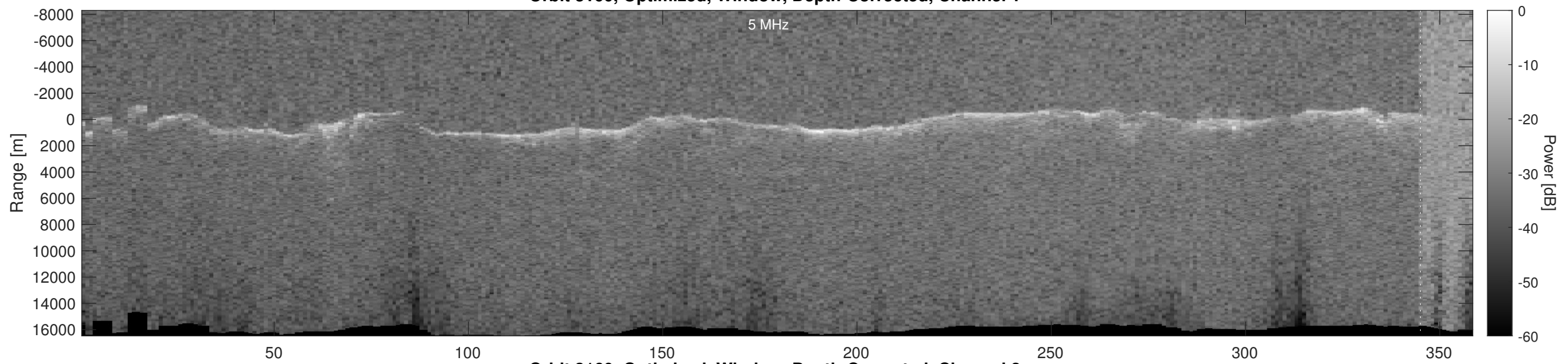
Orbit 3160, Optimized, Window, Depth-Corrected, Channel 2
