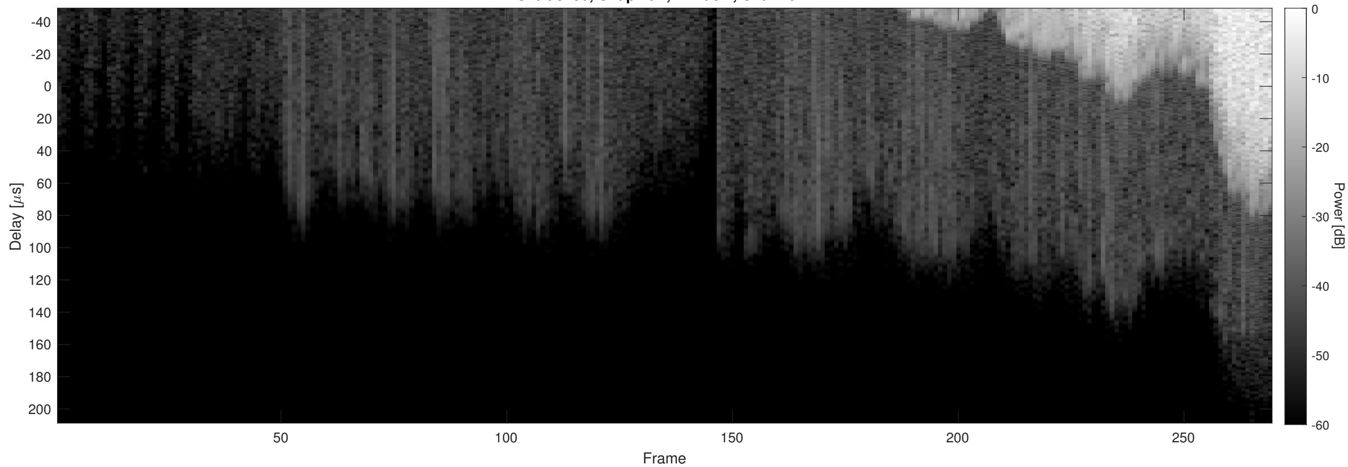
Orbit 3180, Chapman, Window, Channel 2
