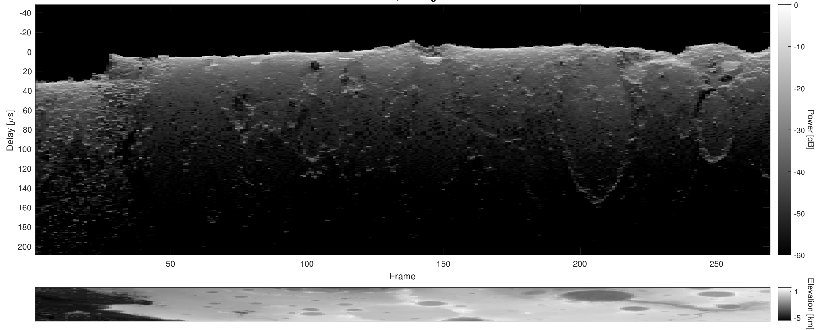
Orbit 3180, Cluttergram
