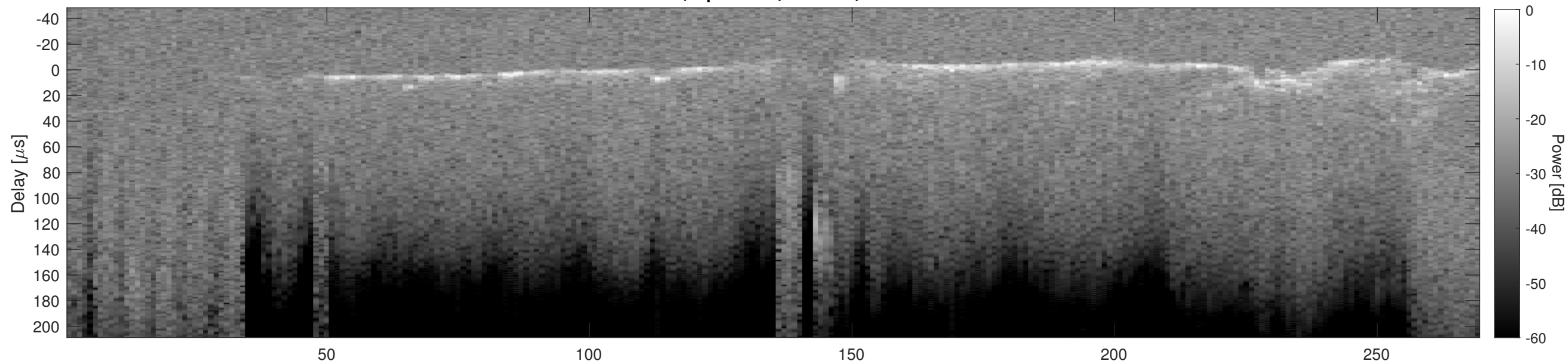
Orbit 3180, Cluttergram
