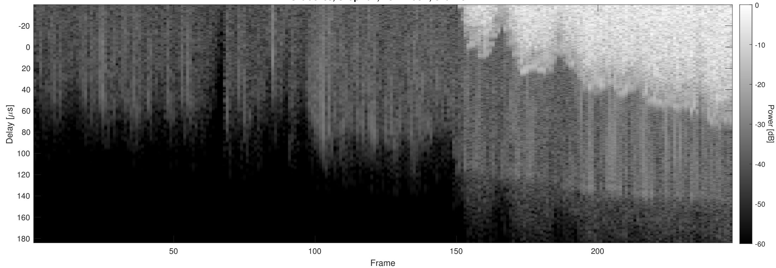
Orbit 3183, Chapman, No Window, Channel 2
