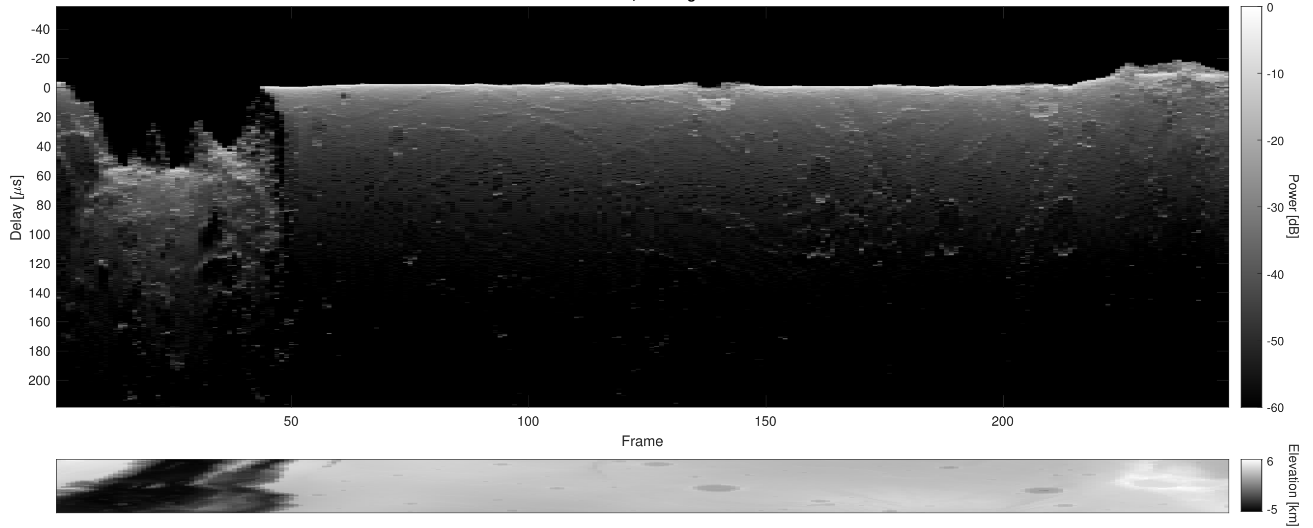
Orbit 3184, Cluttergram
