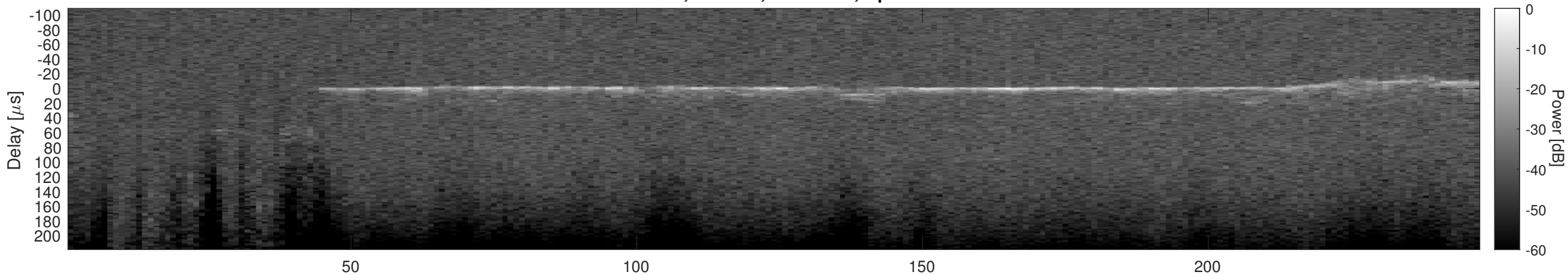
Orbit 3184, Cluttergram
