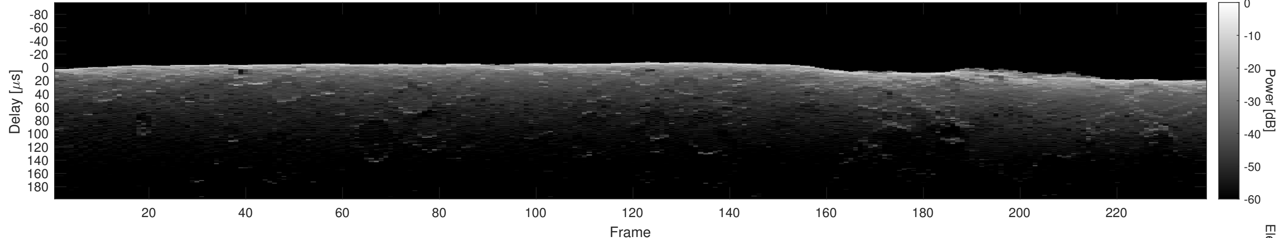
Orbit 3186, Cluttergram
