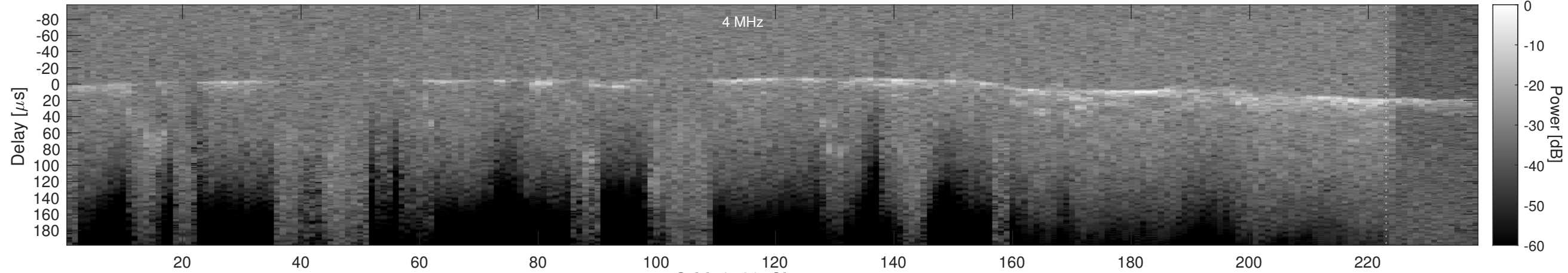
Orbit 3186, Cluttergram
