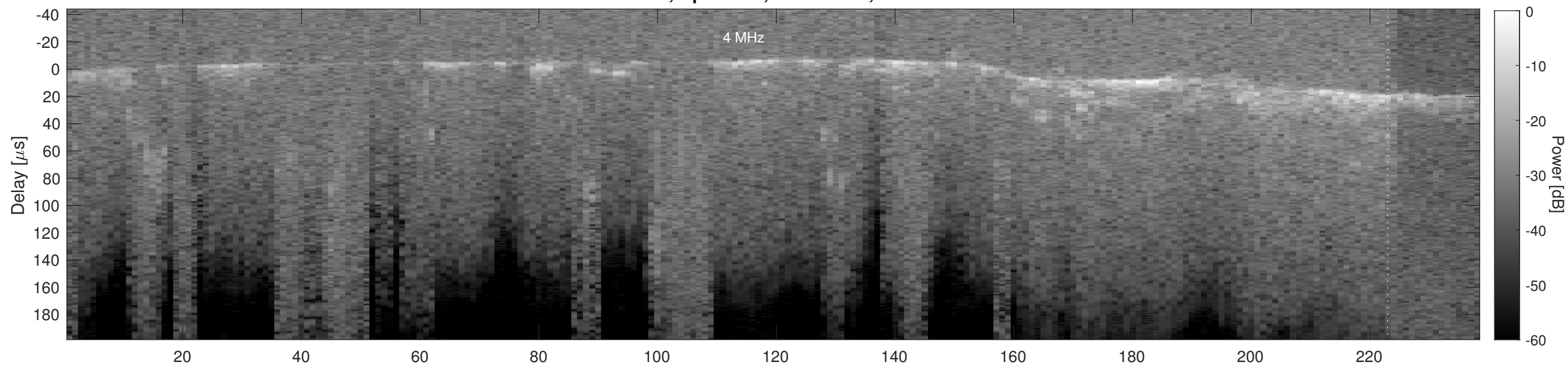
Orbit 3186, Cluttergram
