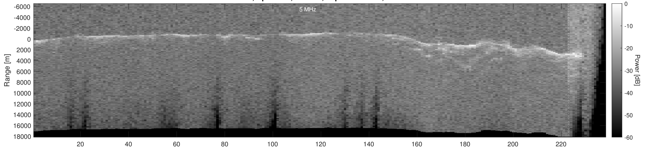
Orbit 3186, Optimized, Window, Depth-Corrected, Channel 2
