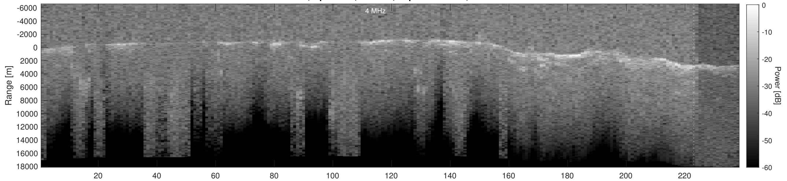
Orbit 3186, Depth-Corrected Cluttergram
