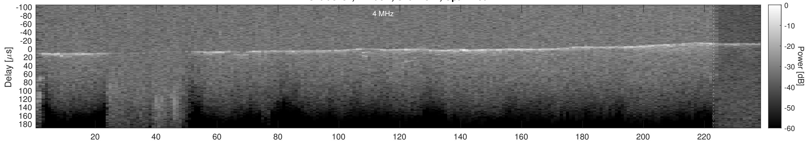
Orbit 3187, Cluttergram
