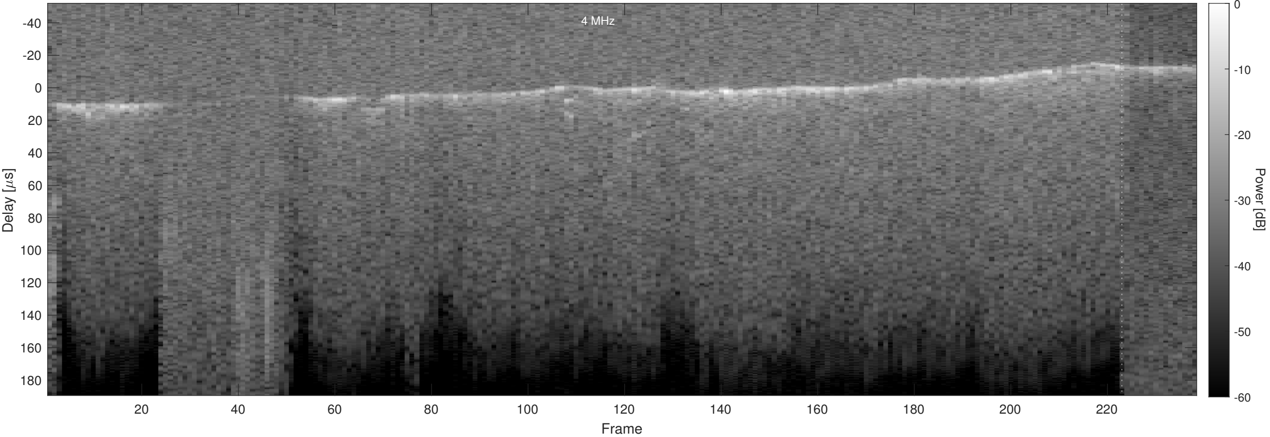
Orbit 3187, Optimized, No Window, Channel 2
