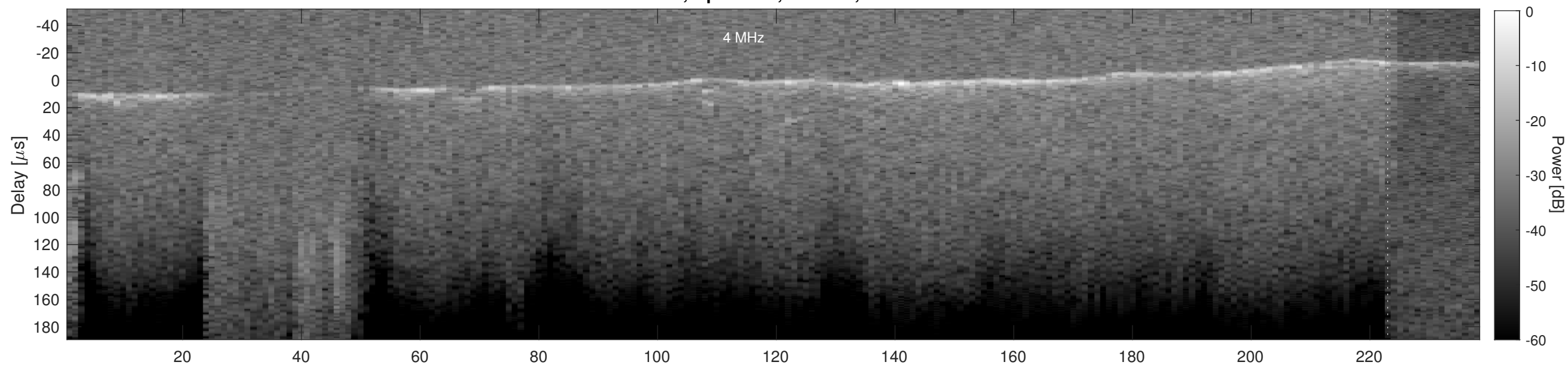
Orbit 3187, Cluttergram
