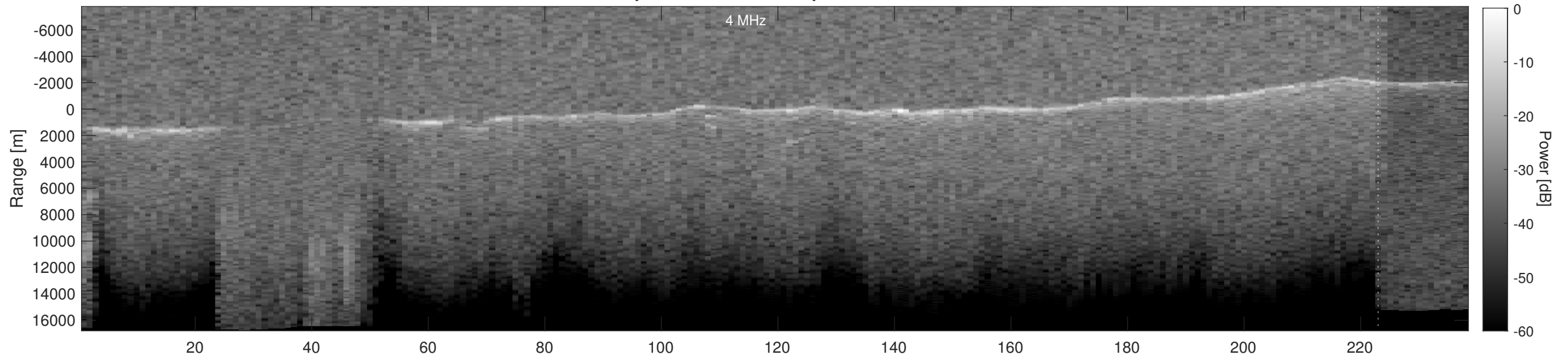
Orbit 3187, Depth-Corrected Cluttergram
