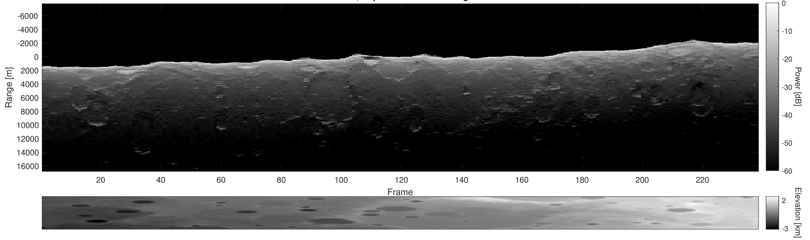
Orbit 3187, Depth-Corrected Cluttergram
