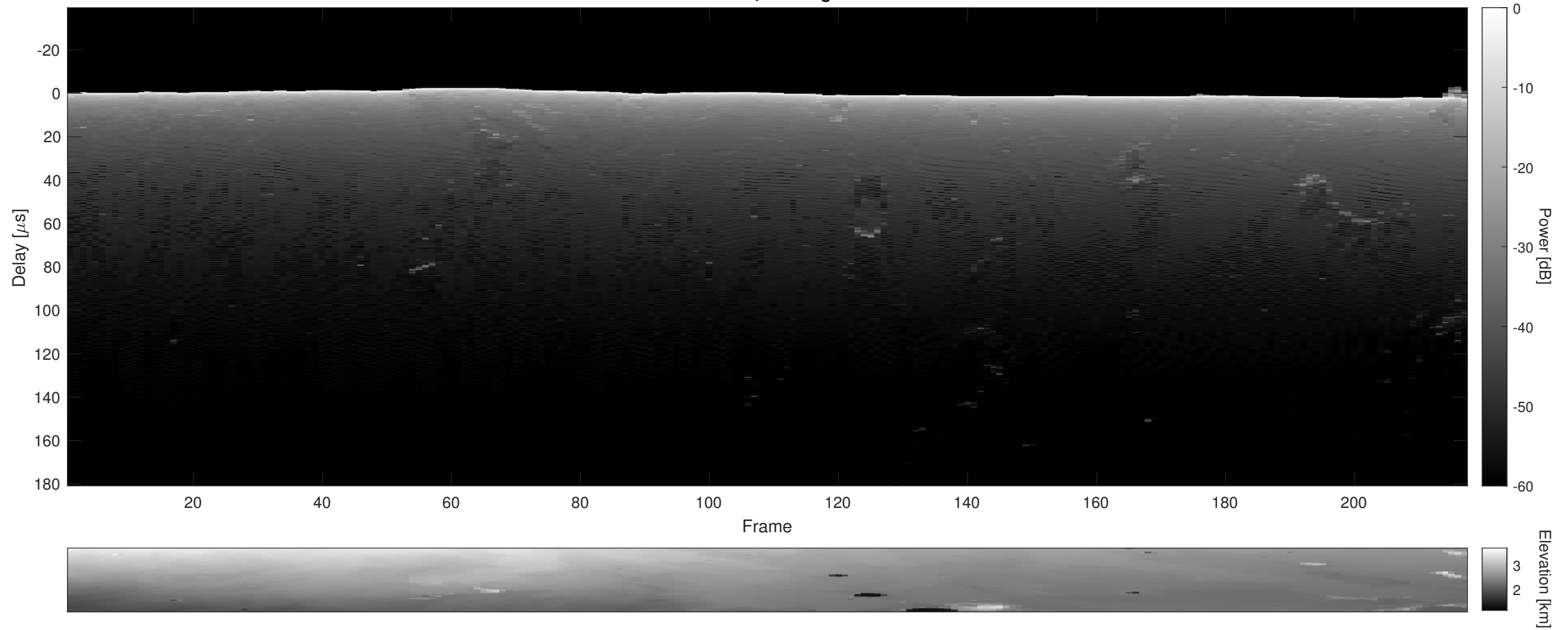
Orbit 3192, Cluttergram
