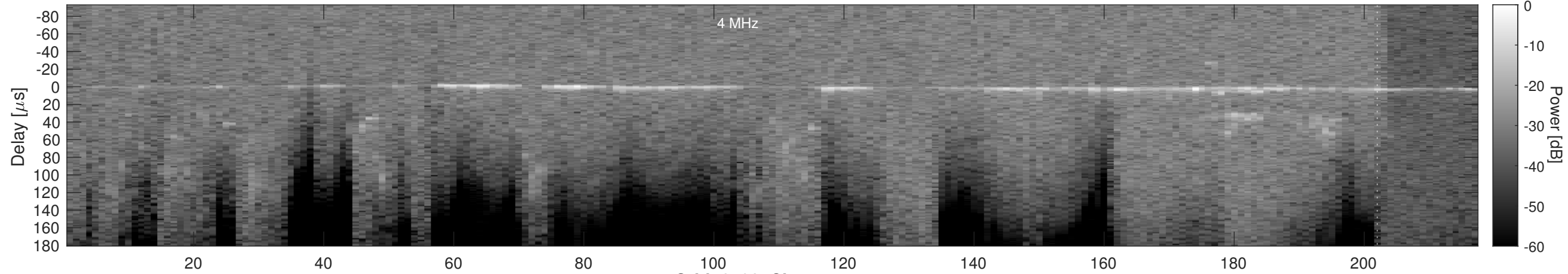
Orbit 3192, Cluttergram
